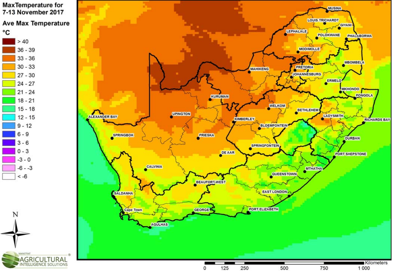
Figure 3: Average Maximum Temperatures, 7-13 November 2017
