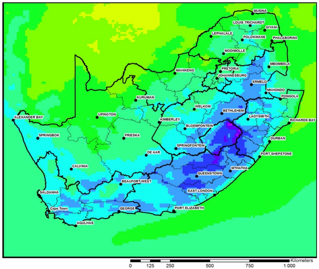
Figure 2: Average Minimum Temperatures, 7-13 November 2017.
