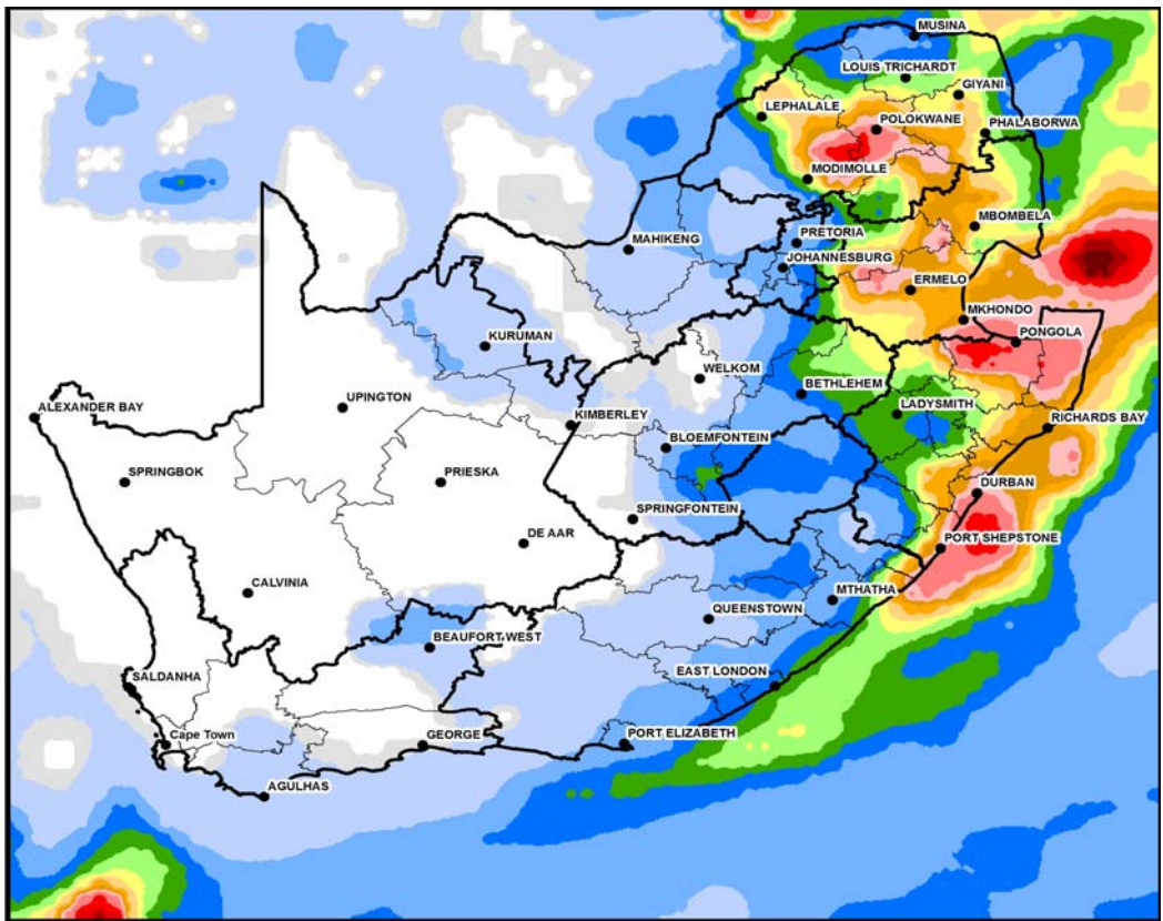
Figure 1: Expected precipitation: 7-13 November 2017.
